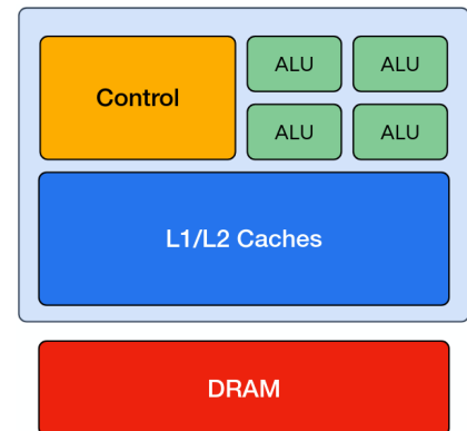
Figure 4.1: Simplified CPU [4]
